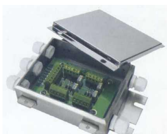
STAINLESS STEEL JUNCTION BOX
